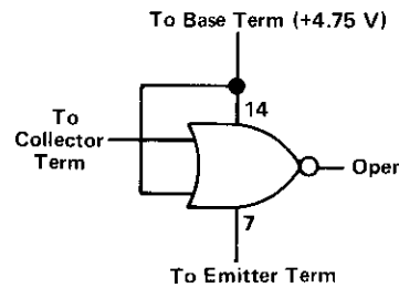
Fig. 51. TTL evaluation, I_{in}(0) condition.
