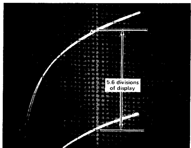
Fig. 20. Display illustrating method of measuring small-signal g_m .
