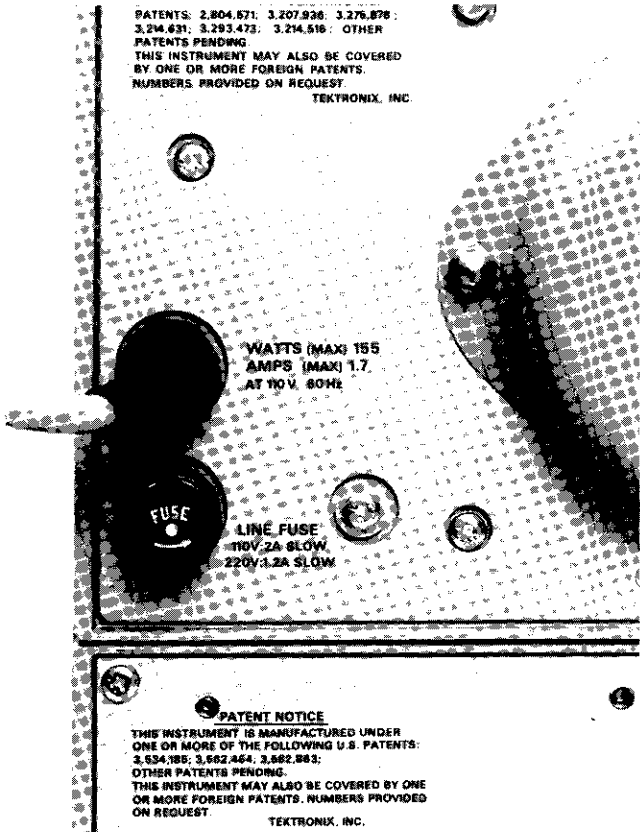
Fig. 1. Fuse location and fuse size information.
