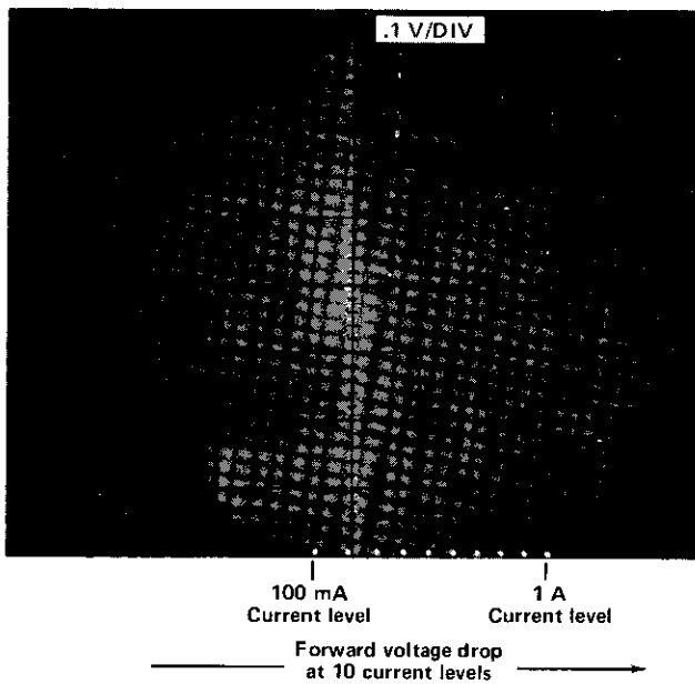
Fig. 29. Display of diode forward drop at high current levels using 300 \mu s PULSED mode.
