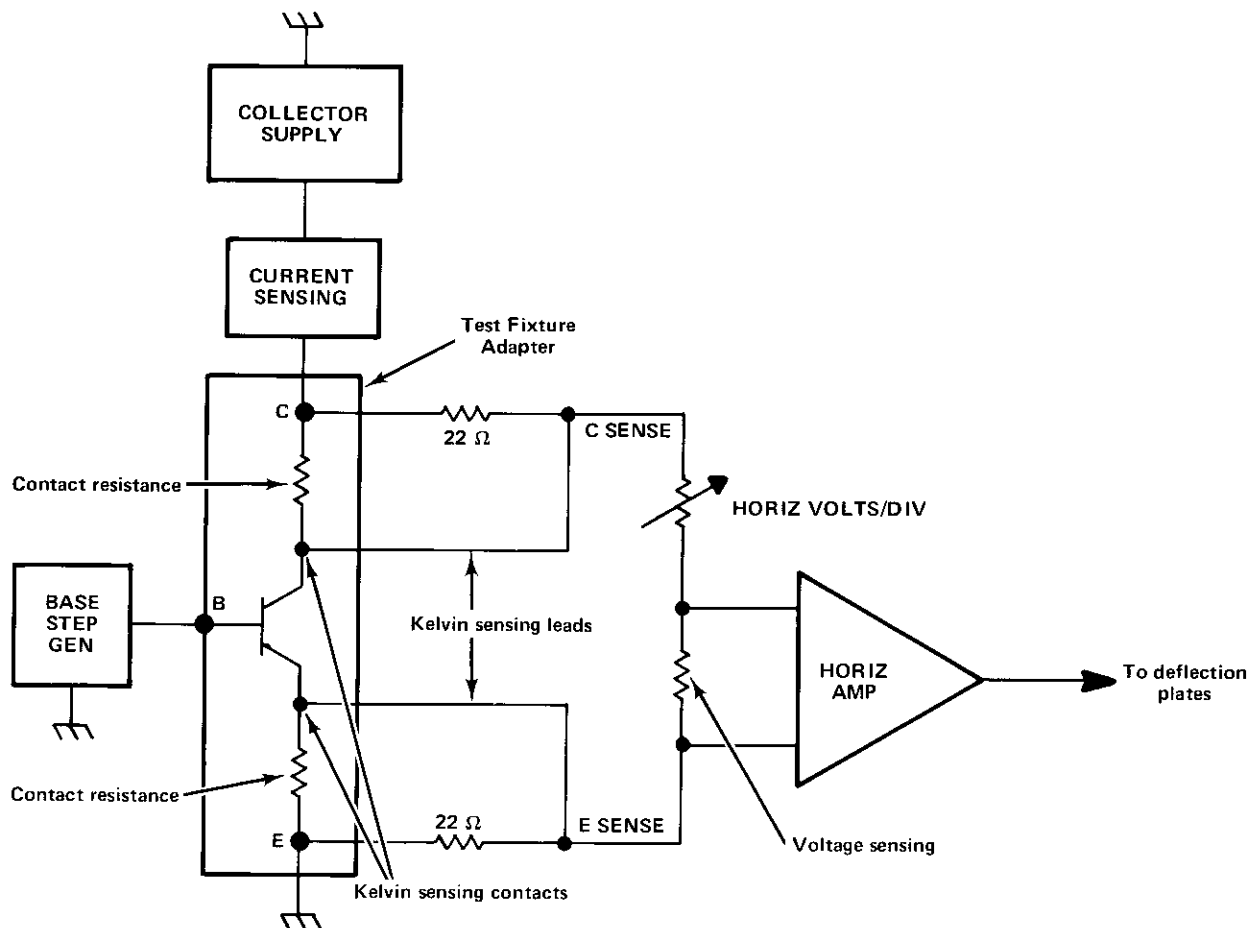
Fig. 4. Kelvin Sensing.
