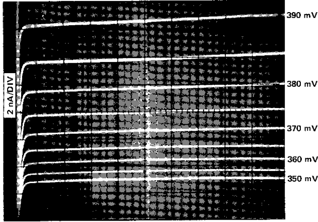
Fig. 18. Characteristics of transistor driven with low base-drive voltage.
